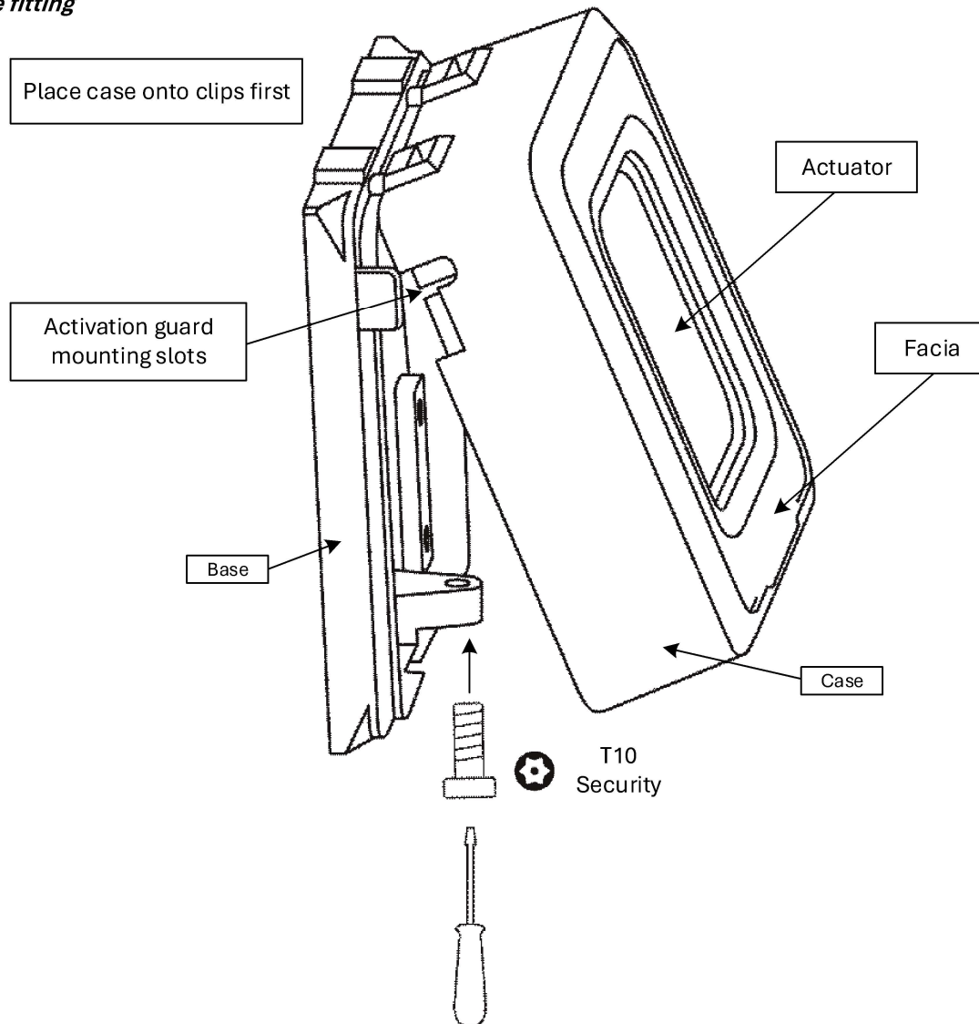
Fig. 3. Case fitting
