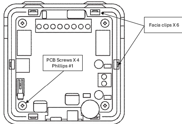
Fig. 5. Facia clips and PCB fixing
