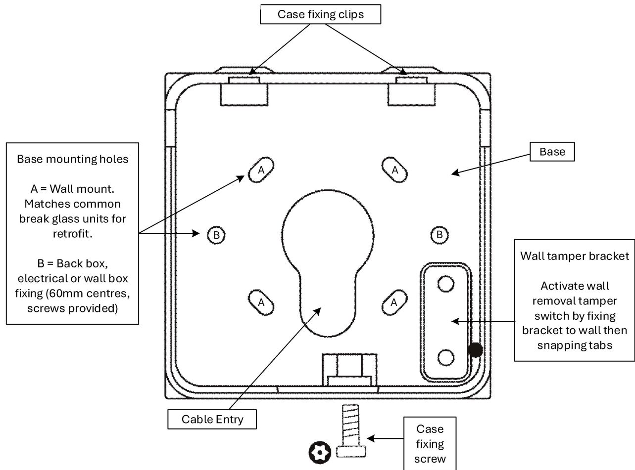
Fig. 2. Base & mounting options
