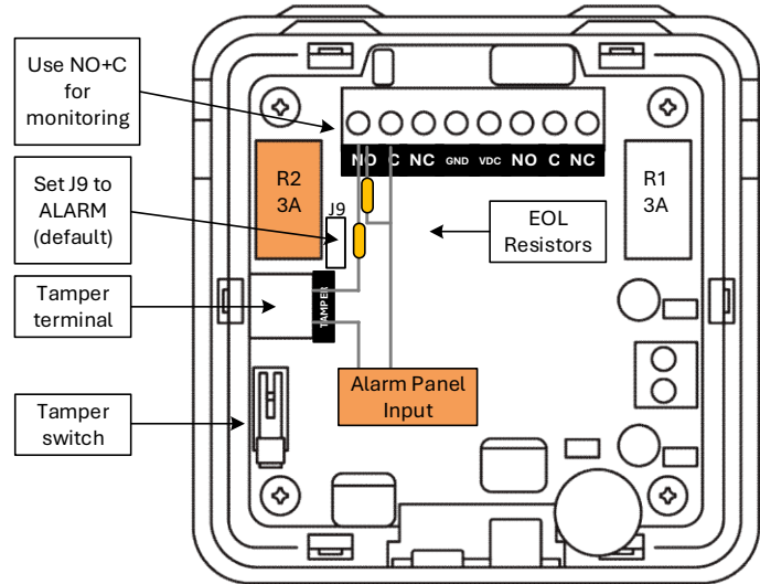
Fig. 12. Series tamper and alarm monitoring
