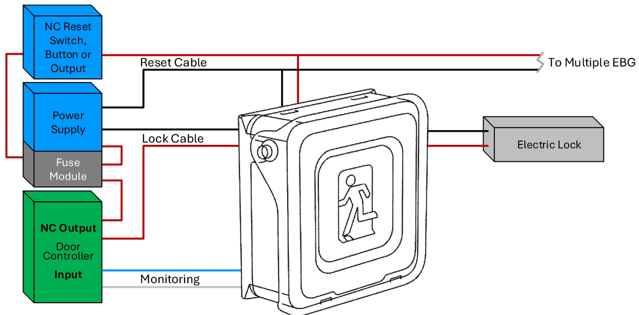
Fig. 18. Dedicated power control, simplified wiring example
