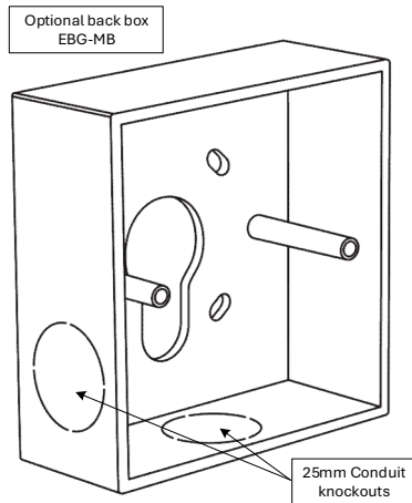
Fig. 4. Optional surface mounting back box
