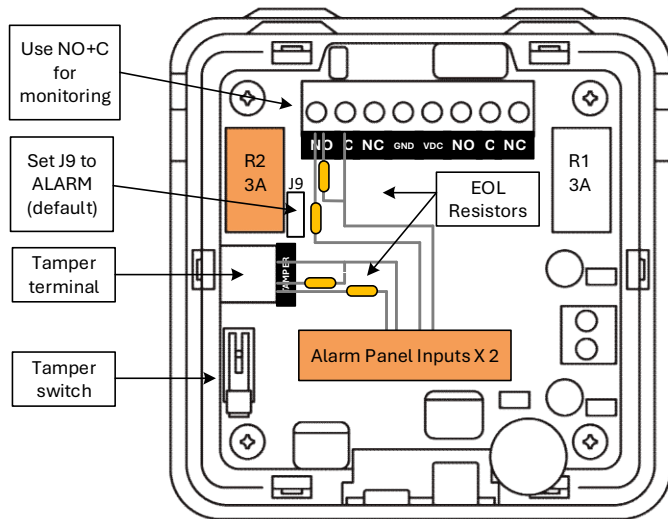
Fig. 13. Separate tamper & alarm monitoring
