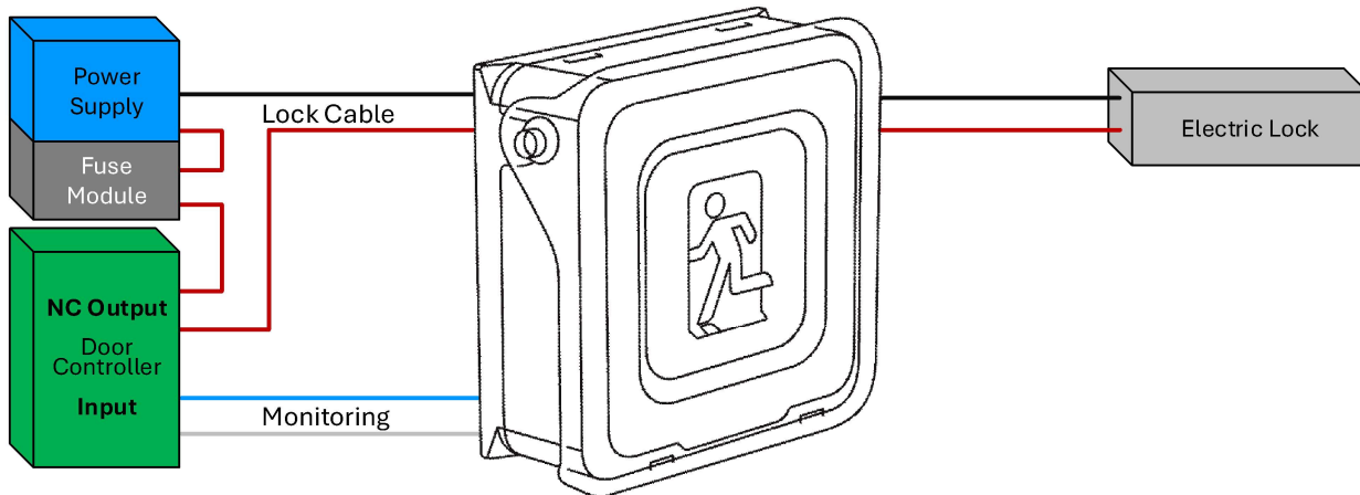
Fig. 17. Lock power control, simplified wiring example
