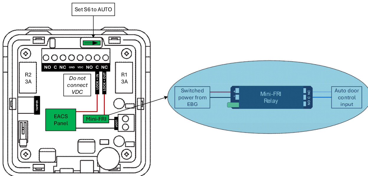
Fig. 10. Auto door with relay interface
