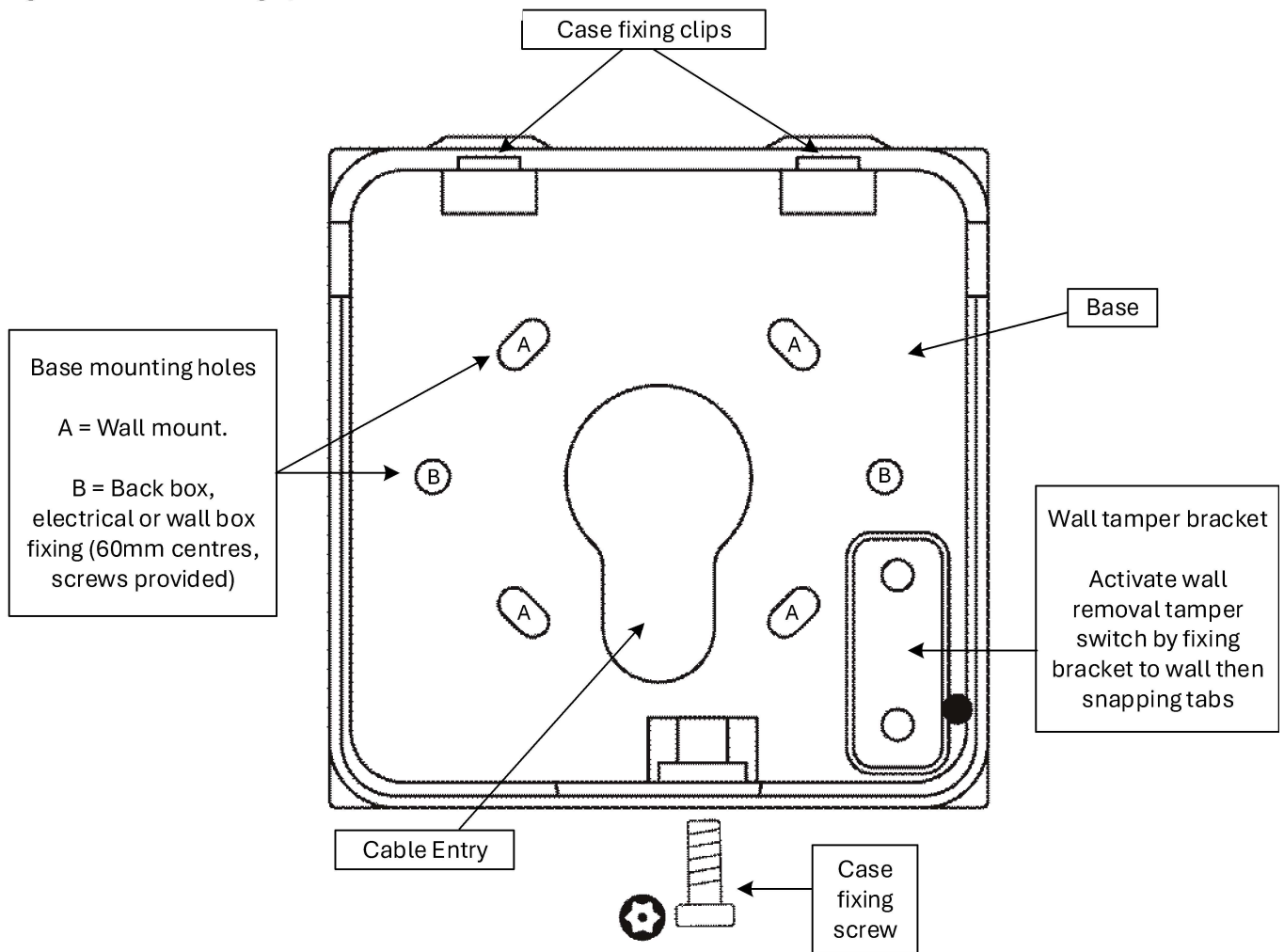
Fig. 6. Base & mounting options
